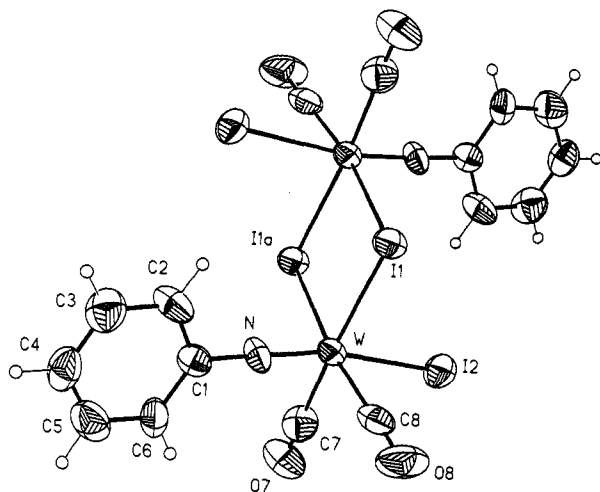
Figure 1. ORTEP drawing of compound 2 ·0.5H 2 O showing the crystallographic numbering scheme. Hydrogen atoms and the partial solvent molecule are omitted. Thermal ellipsoids are drawn at the 40% probability level. Selected distances (Å) and angles (deg) are as follows: W–I1 2.826(1), W–I1a 2.829(1), W–I2 2.808(1), W–N 1.756(10), W–C7 2.051(14), W–W 4.239(1), W–N–C1 177.0(8), I1a–W–I1 82.90(3), I1–W–N 97.0(3), I2–W–N 170.0(3), I1a–W–C8 170.3(4).
